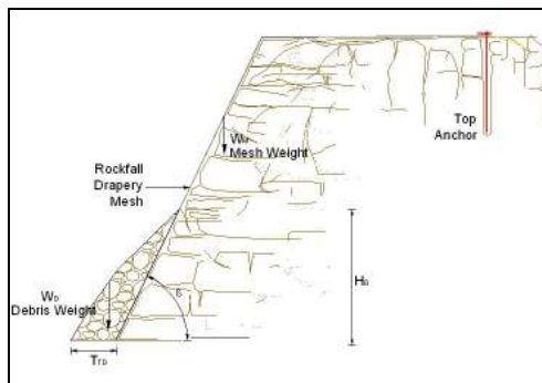
Figure 10. Conceptualisation of a drapery system
